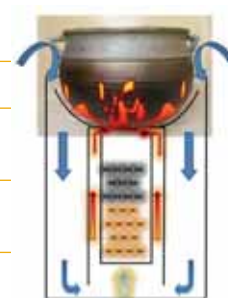
Photo 4.26 AARON stove
